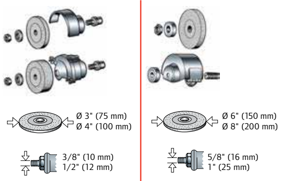
Type 1 Wheels
